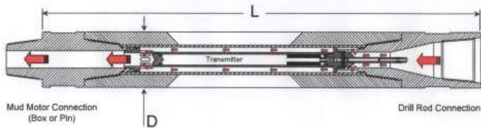
High Flow Sonde Housing - Digitrak™ 2 & 4 Battery & Eclipse
